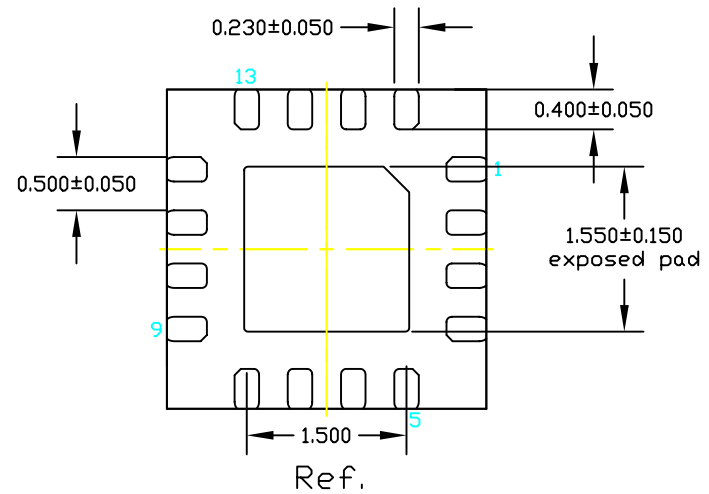
Btm View
