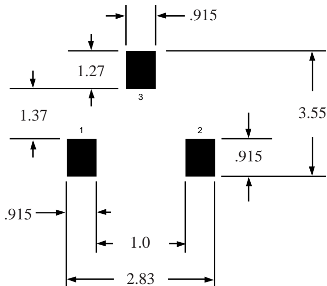
PC Board
