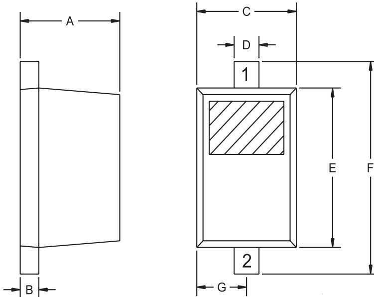
SOD523 Flat Lead -OUTLINE Drawing
