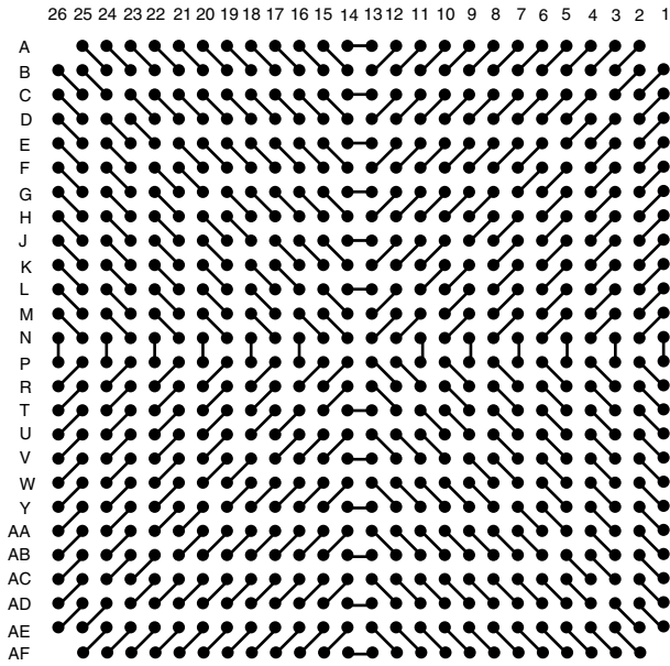
BALL VIEW
