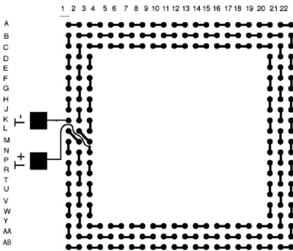
Test Vehicle Board
