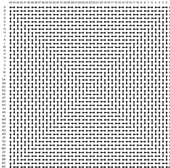
BALL VIEW
