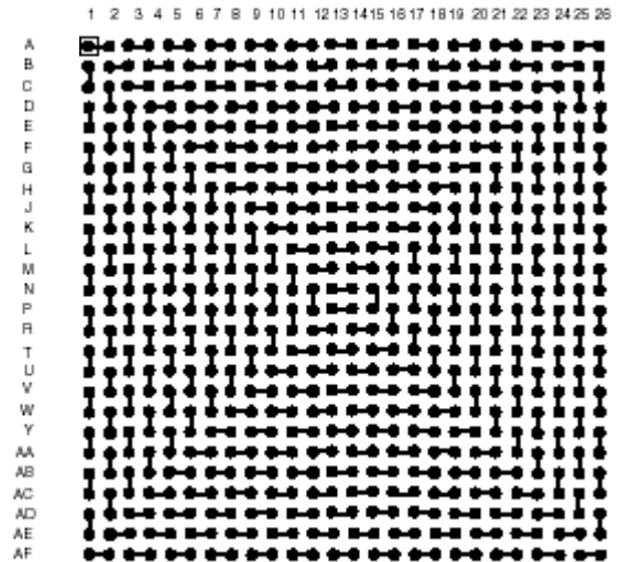
BOTTOM SIDE (TOP X-RAY VIEW)
